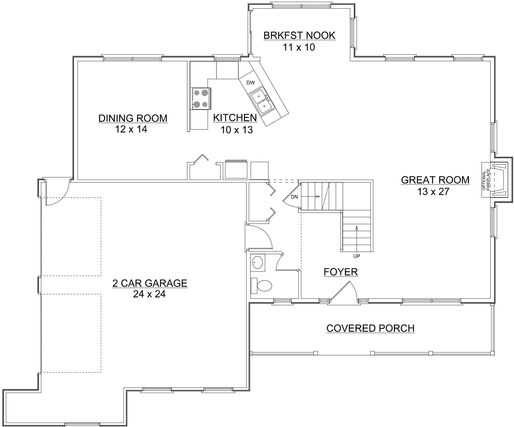
MAIN FLOOR PLAN
